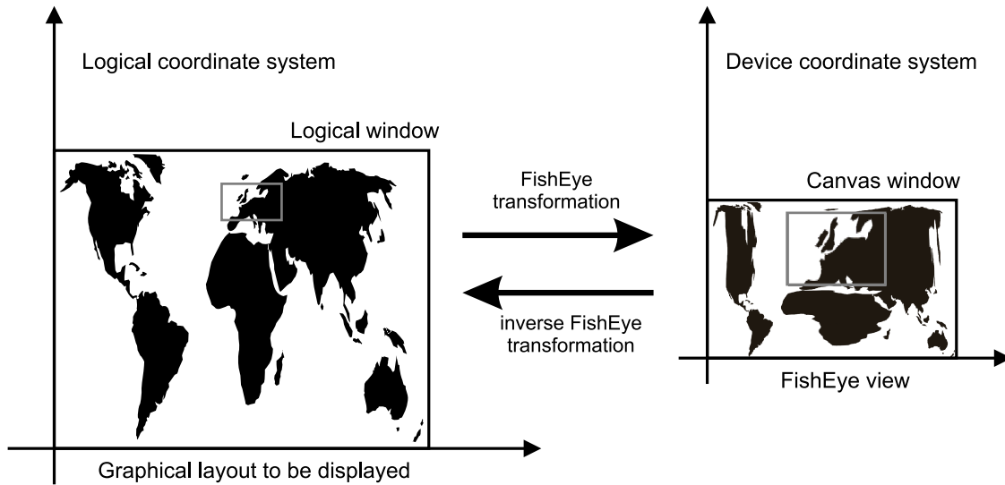
Figure 1: Illustration of the fisheye transformation.
