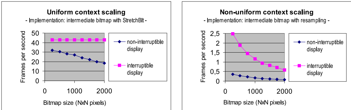
Figure 5: Display refresh rates 2 of the implementation using an intermediate bitmap. Left: Uniform scaling by StretchBlt operation of graphical subsystem. Right: Non-uniform scaling by Fant's resampling algorithm.
