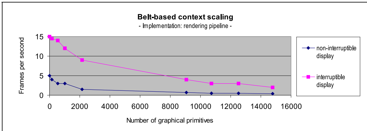
Figure 7: Display refresh rates 3 of the implementation using the rendering pipeline of the graphical subsystem.
