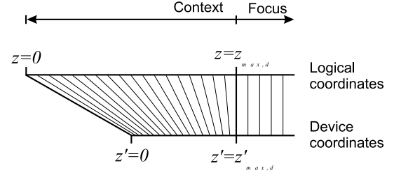
Figure 4: The idea of non-uniform context scaling.
