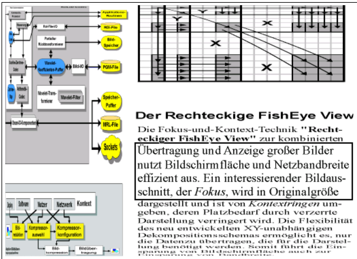
Figure 6: RECTANGULAR FISHEYE VIEW displaying a 2D vector graphics layout using a 1024x713 pixel background bitmap and non-uniform context scaling with \epsilon = 1.5 . Canvas window size: 512x357 pixels.
